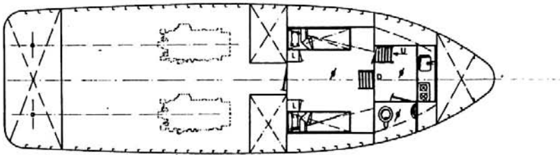
VIEW BELOW MAINDECK
