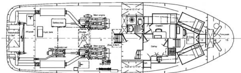
Below Maindeck
